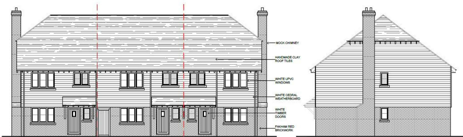
FRONT ELEVATION - 1 : 1 0 0
